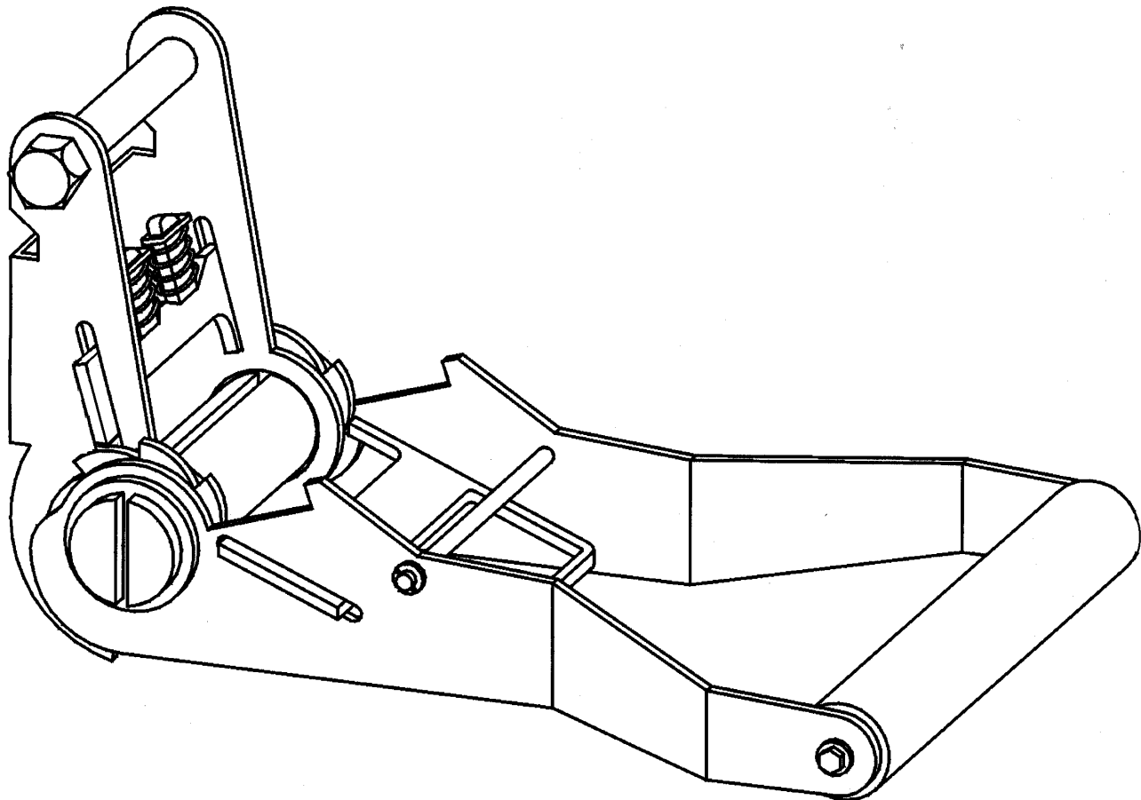
Figure 4 — Crossbar type ratchet
