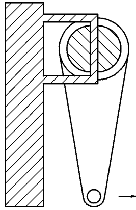
Figure 8 — Positioning for strength test of the handle
